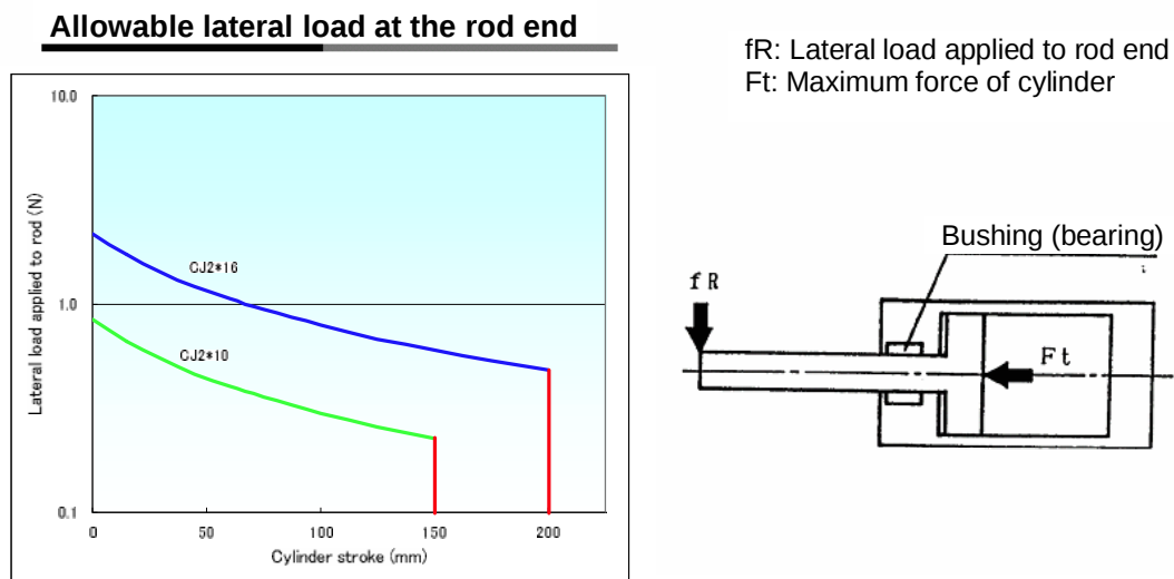
Fig. 1 Allowable lateral load applied to rod end
