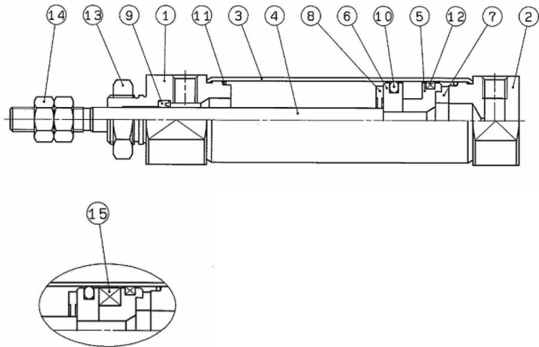
Fig. 4 Standard product: Double acting/single rod
