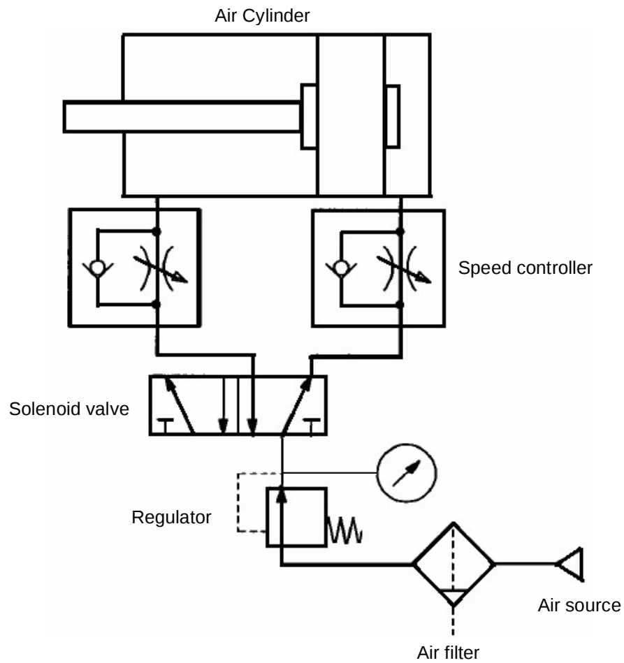
Fig.3 Basic Circuit
