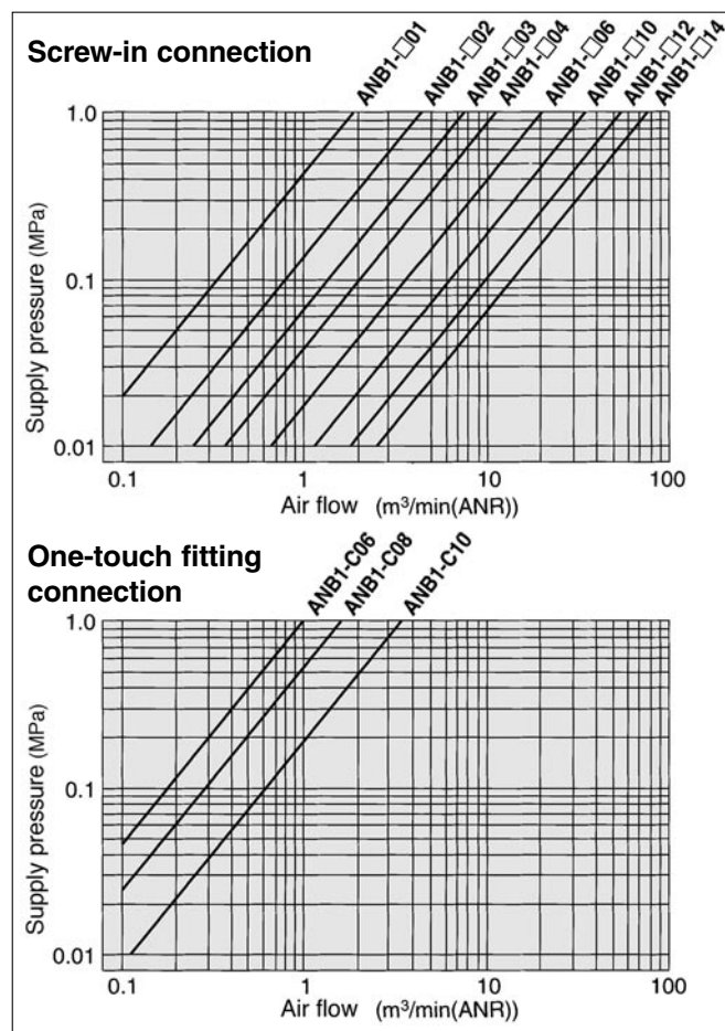
Flow Characteristics/ANB1 (Initial conditions)
